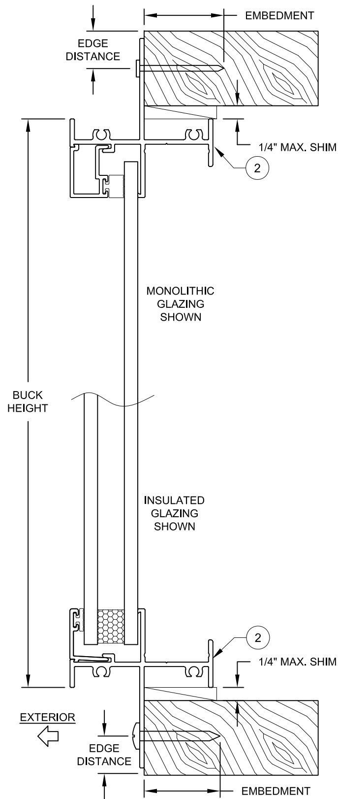
VERTICAL SECTION D-D
